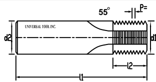
WITH WORTH BSW & BSF
