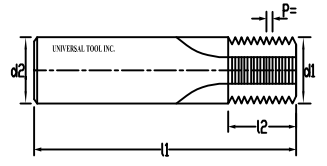
UNF
