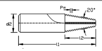
20 TAPER THREAD MILL \alpha = 60^\circ & \alpha = 55^\circ
