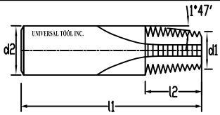
NPT
