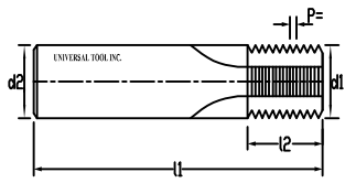
ISO METRIC (Fine Thread)
