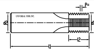
BSPT
