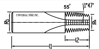
BSPT
