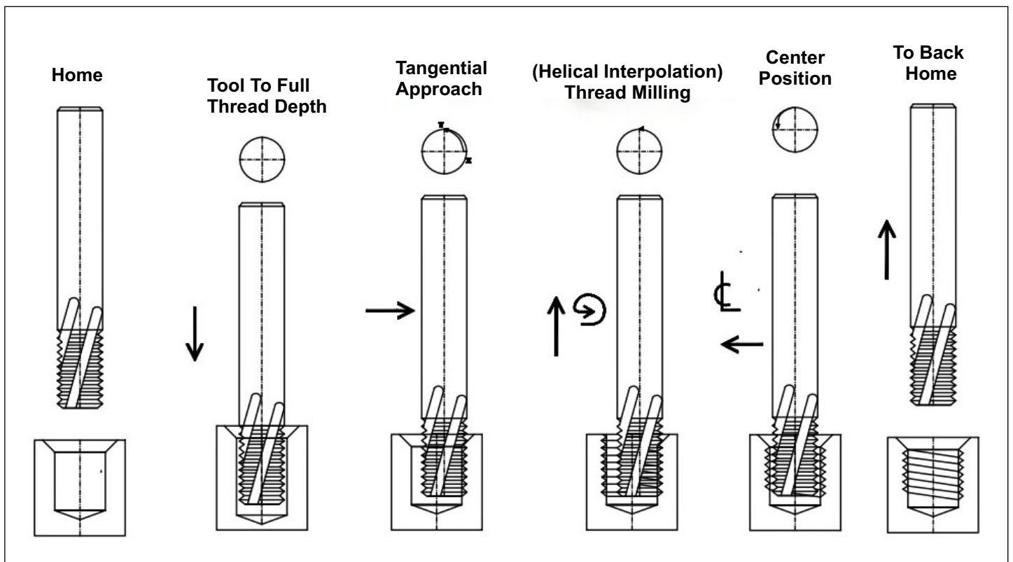
20 TAPER THREAD MILL \alpha = 60^\circ & \alpha = 55^\circ
